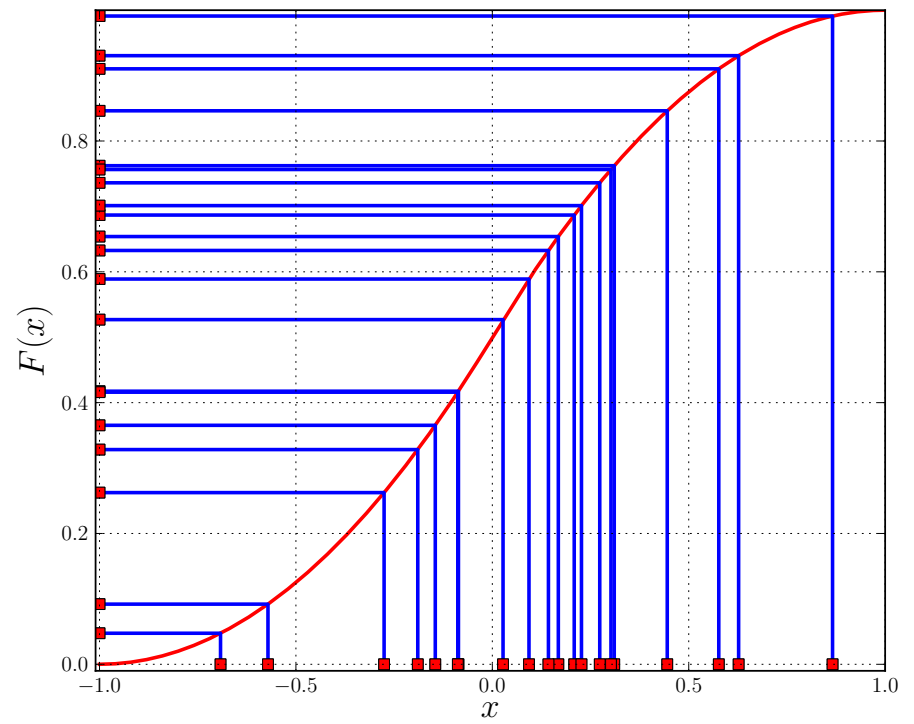
The "Tent" distribution function.
